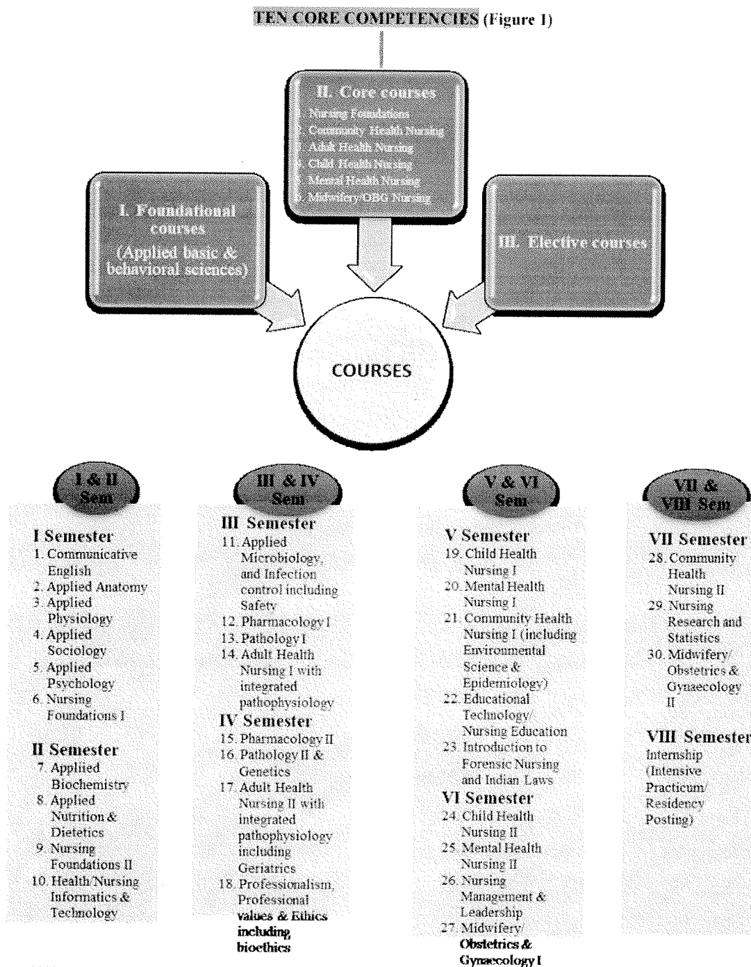
Figure 2. Curricular Framework
